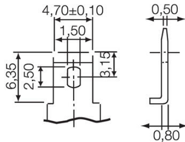
Faston flat connector 4,8 mm
