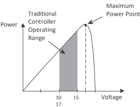
Output Power (12V System)
