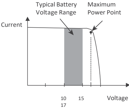
Current vs. Voltage (12V System)
