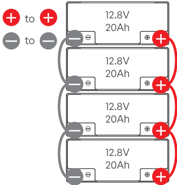
Parallel Connection 12V(12.8V) 80Ah
