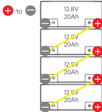
Series Connection 48V(51.2V) 20Ah
